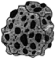
A Conglomerate
